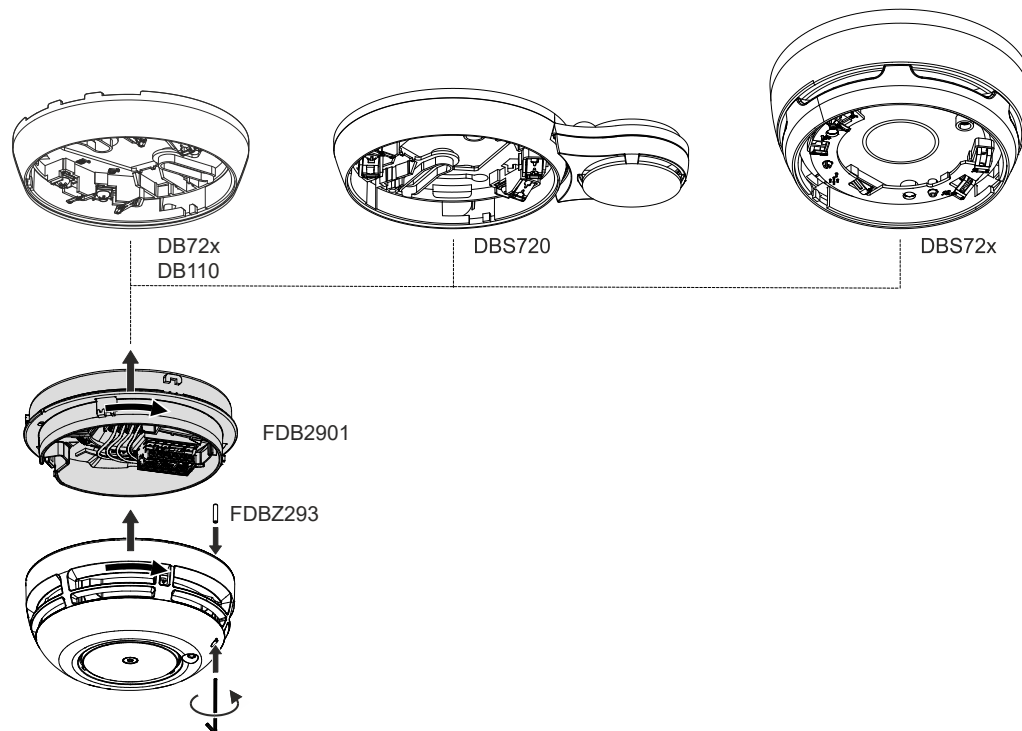
Fig. 1: Installing FDB2901 base adapters
